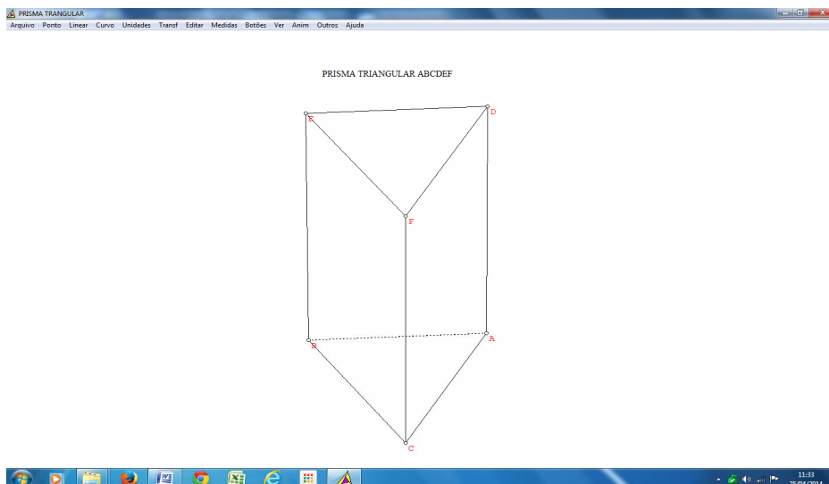
Figura 4: prisma triangular
