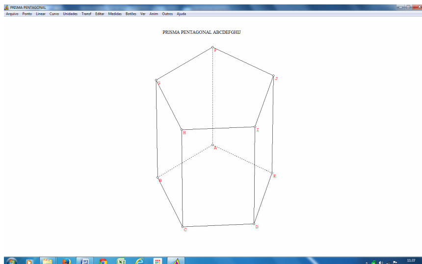
Figura 6: prisma pentagonal.
